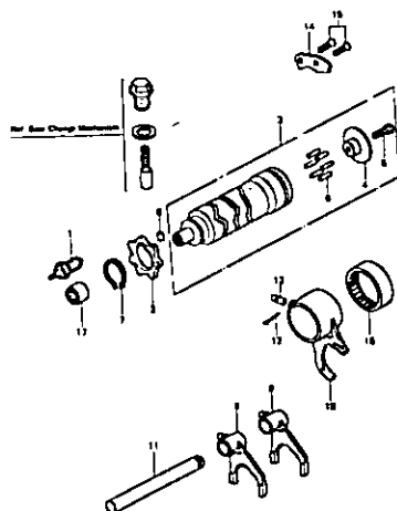
11. Change Drum, Shift Fork ..... 12
