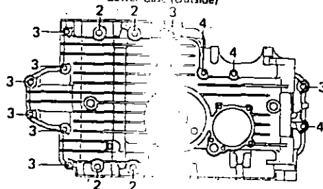
Lower Case (Outside)
