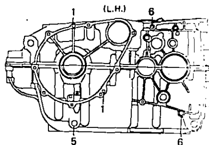
Lower Case (Outside)
